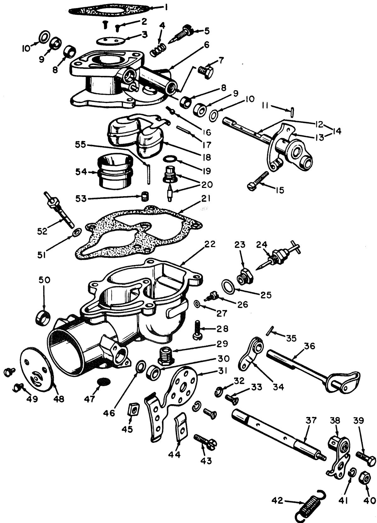
Fig. 6. Exploded View
