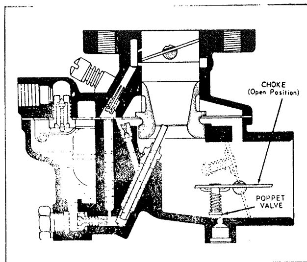
Fig. 5. Choke System
