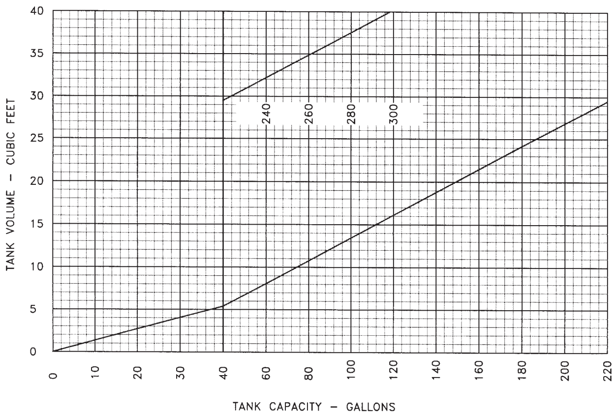
FIGURE 3 Tank Volume
